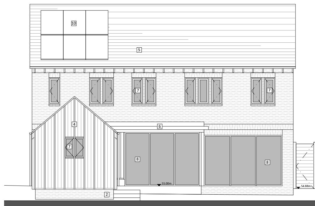
REAR (SW) ELEVATION
