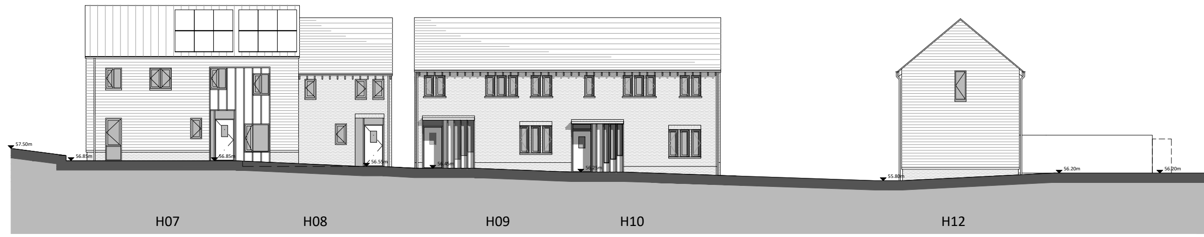
50.00m AOD SITE SECTION C - C
