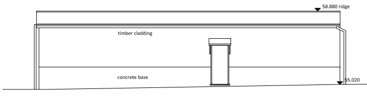
Unit D South West Elevation
