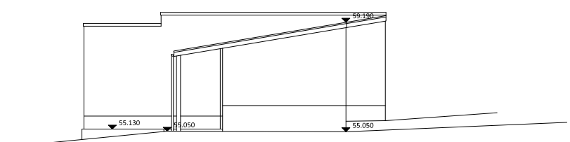
Unit F South East Elevation
