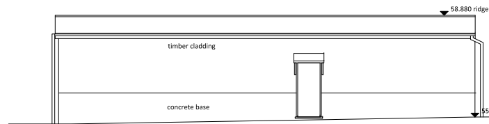
Unit D South West Elevation
