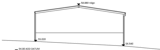
Unit D North West Elevation
