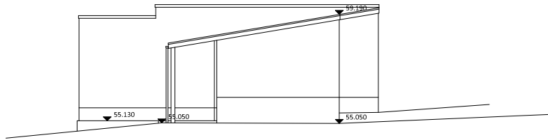
Unit F South East Elevation
