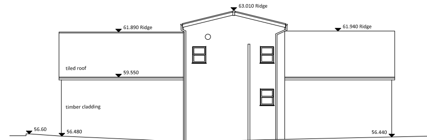
Unit B North East Elevation
