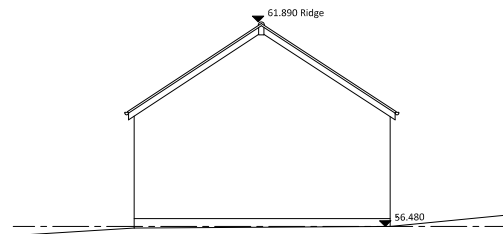
Unit B South East Elevation
