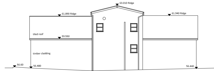
Unit B North East Elevation
