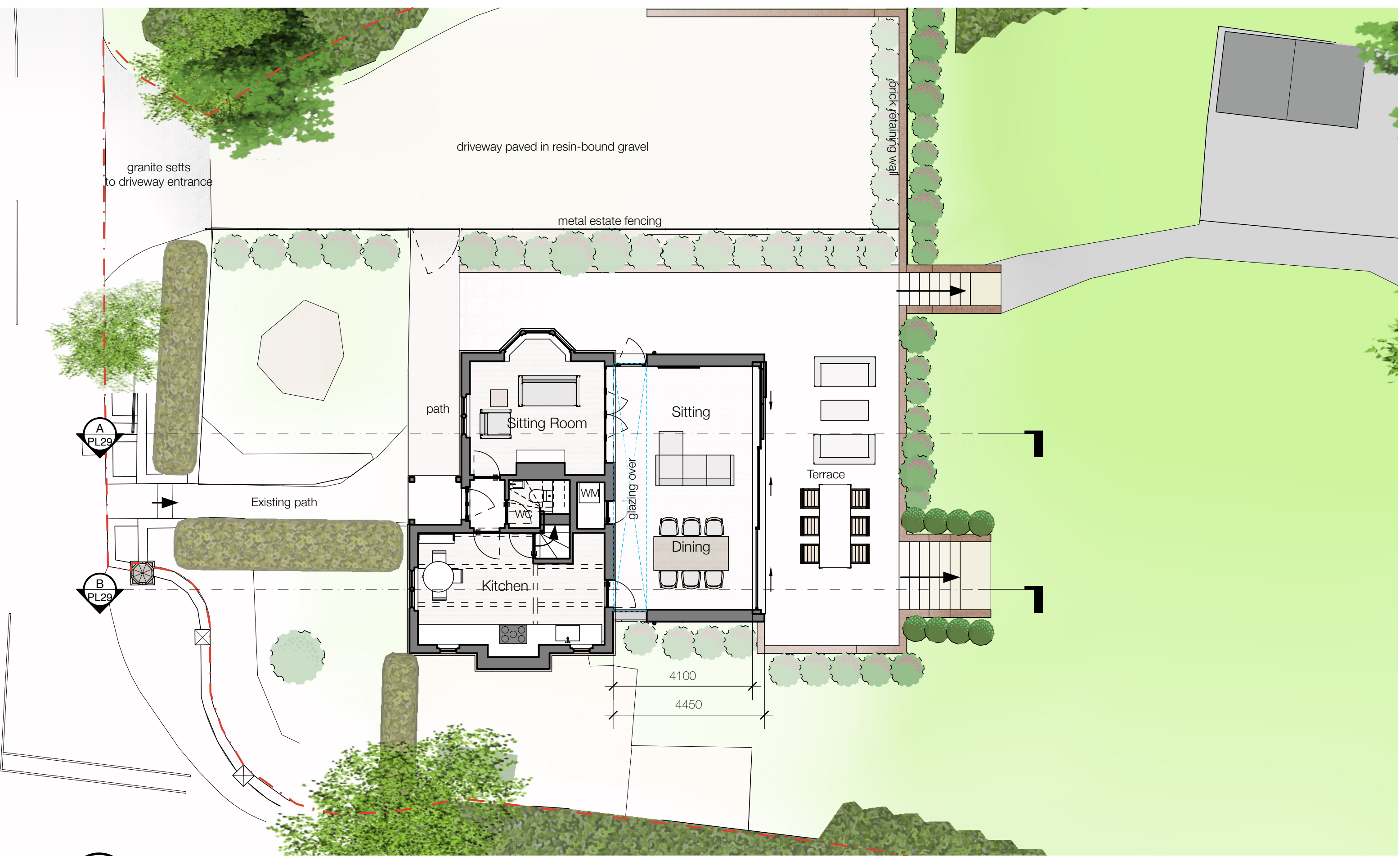
A Proposed Ground Floor Plan PL11 1:100
