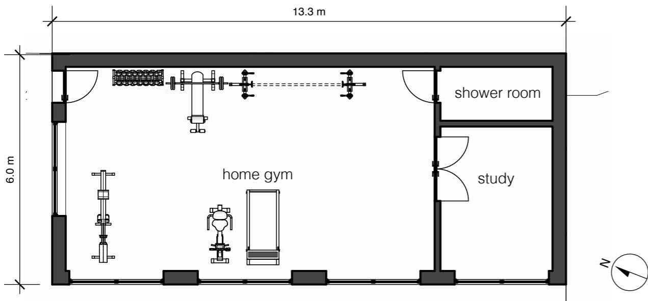
A Floor Plan 1:100
