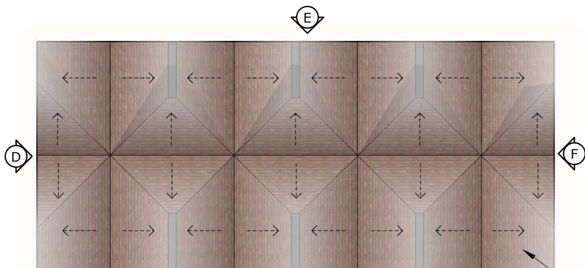
B Roof Plan 1:100
