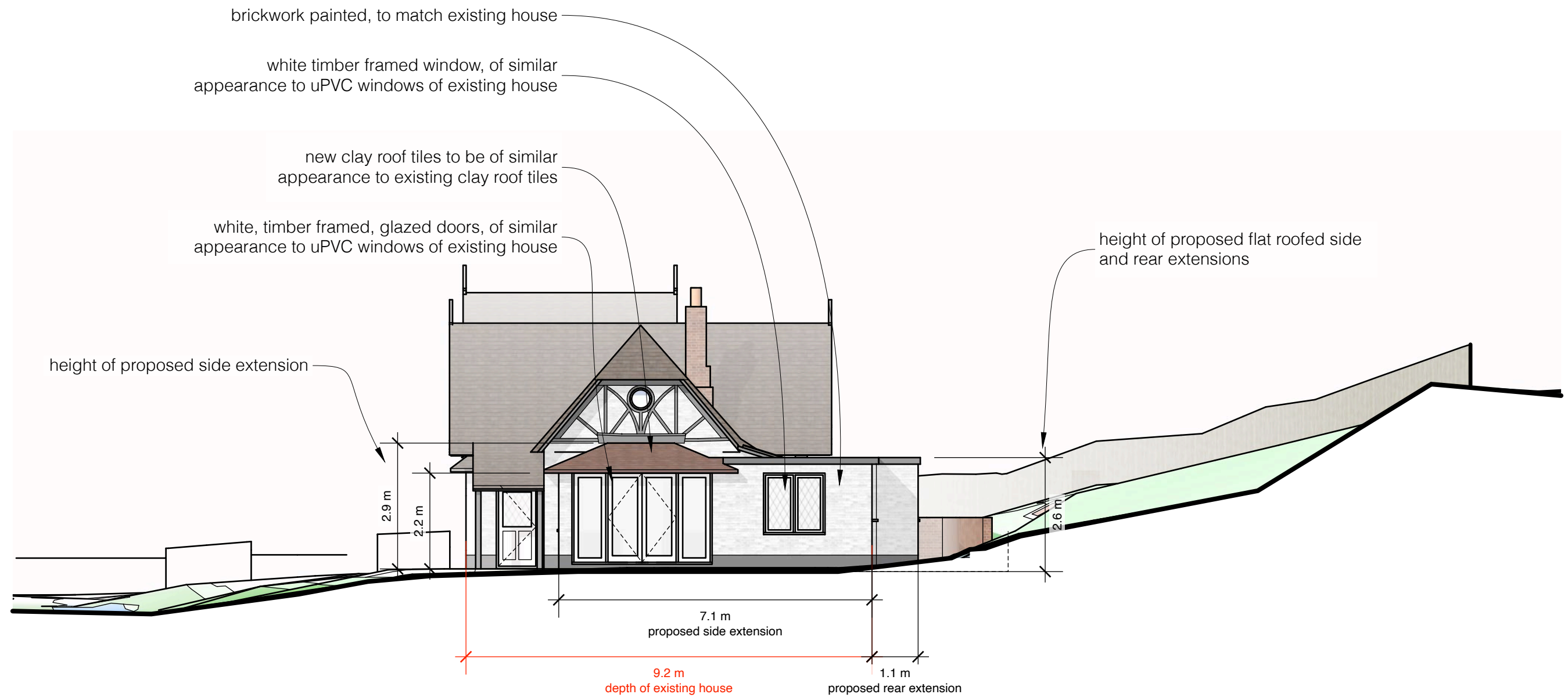
A Proposed Side Elevation (South) PD17 1:100
