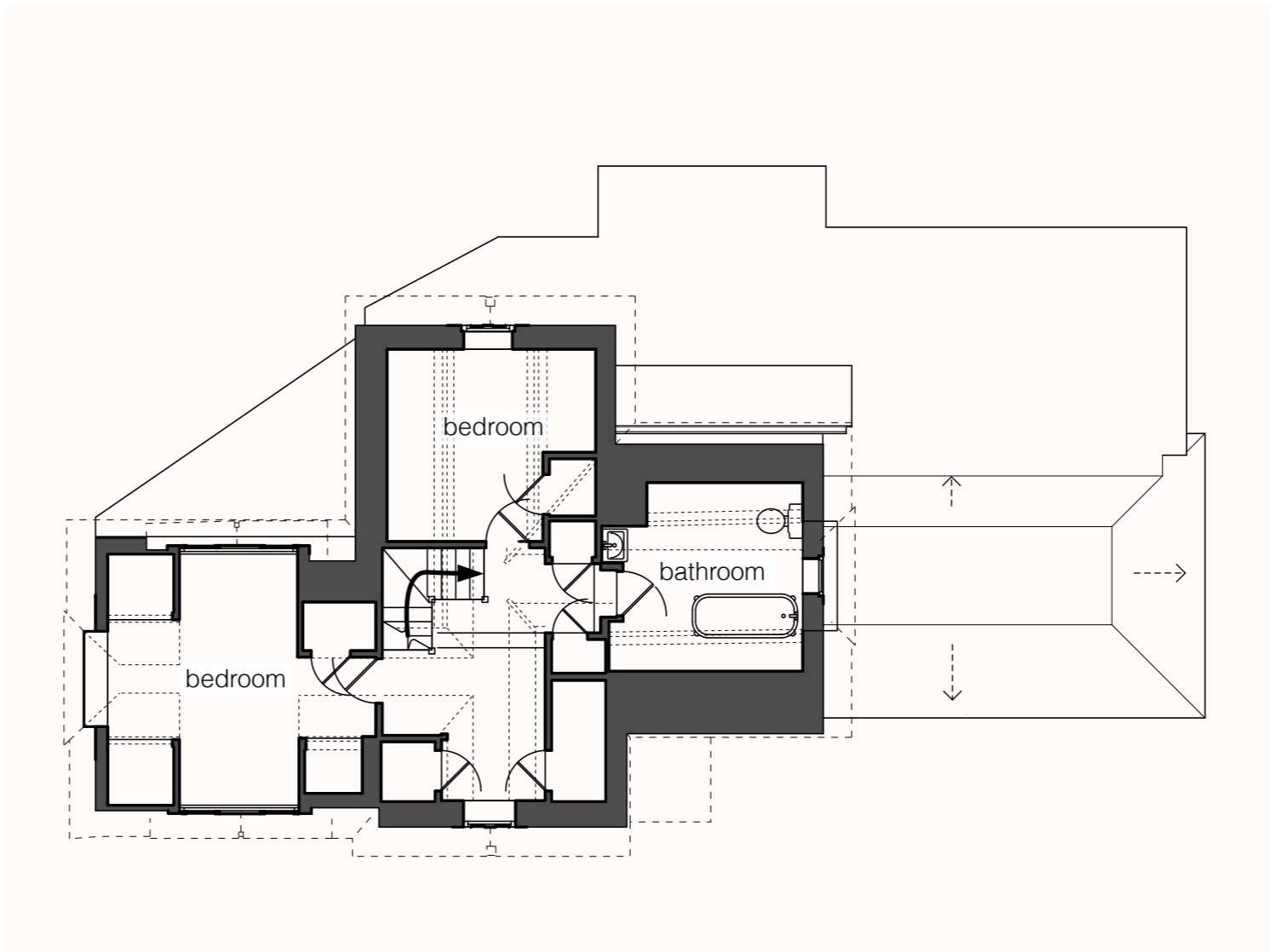
A Proposed First Floor Plan PD14 1:100
