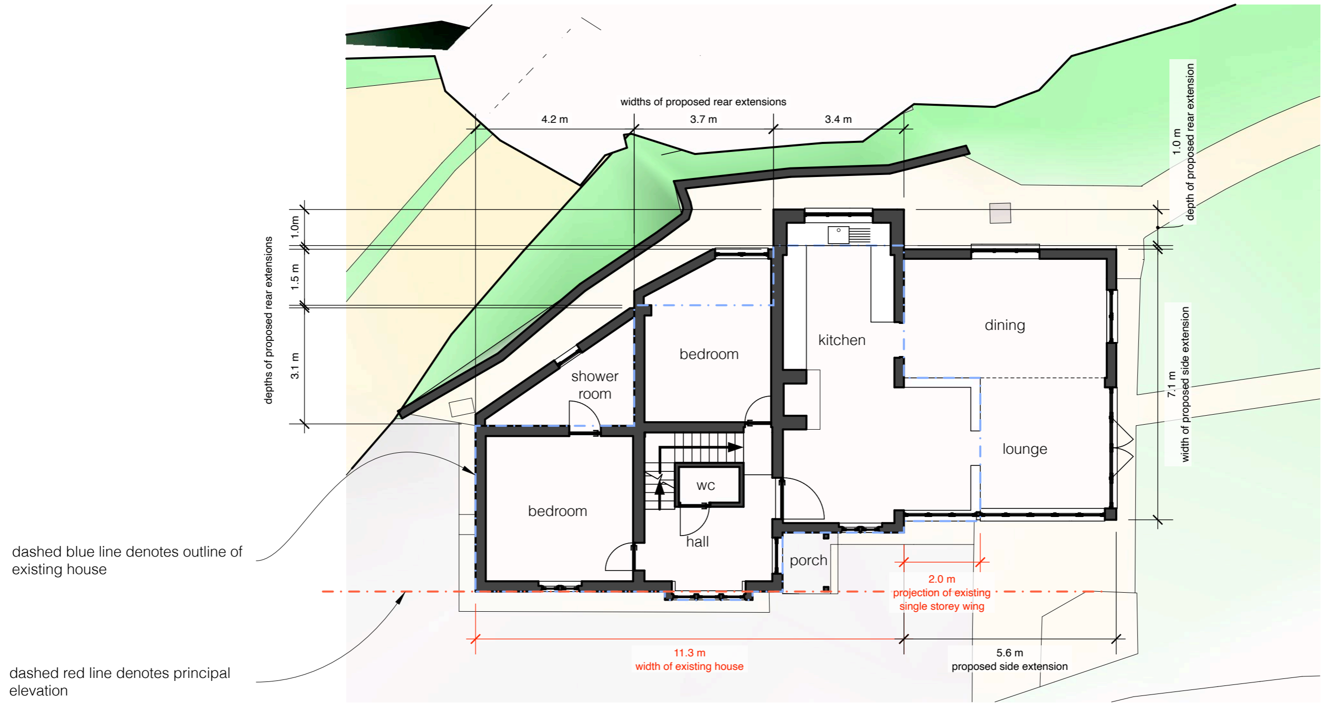
A Proposed Ground Floor Plan PD13 1:100
