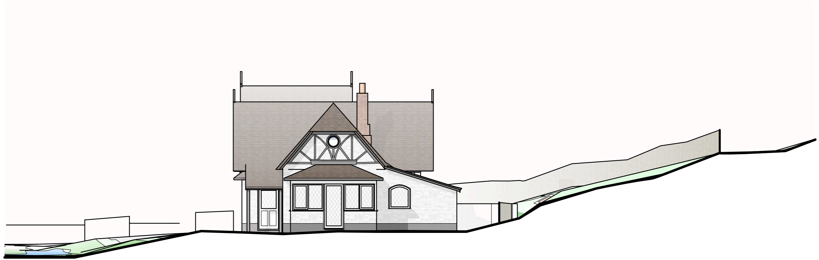
A Existing Side Elevation (South) PD08 1:100
