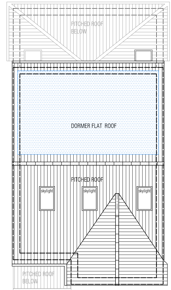
[04] PROPOSED ROOF PLAN
