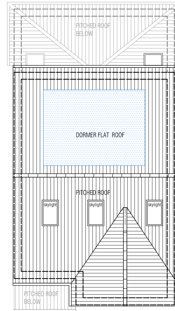
[04] PROPOSED ROOF PLAN
