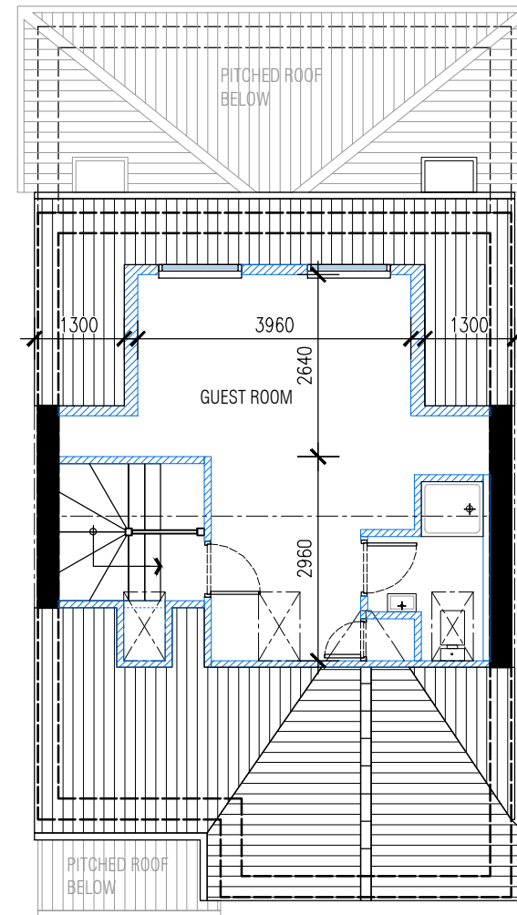
[03] PROPOSED LOFT PLAN
