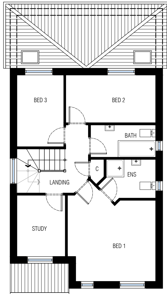
[02] PROPOSED FIRST FLOOR
