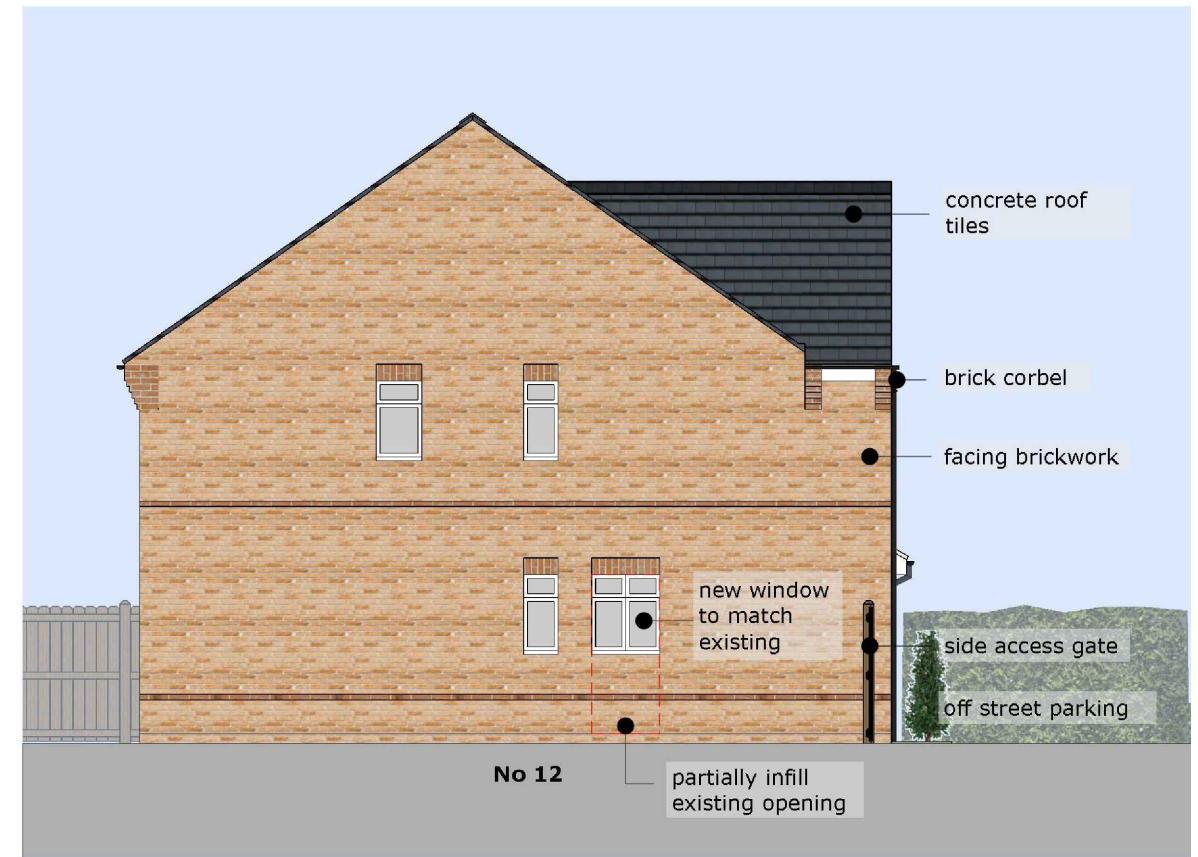
[03] PROPOSED SIDE ELEVATION (EAST) 1:100
