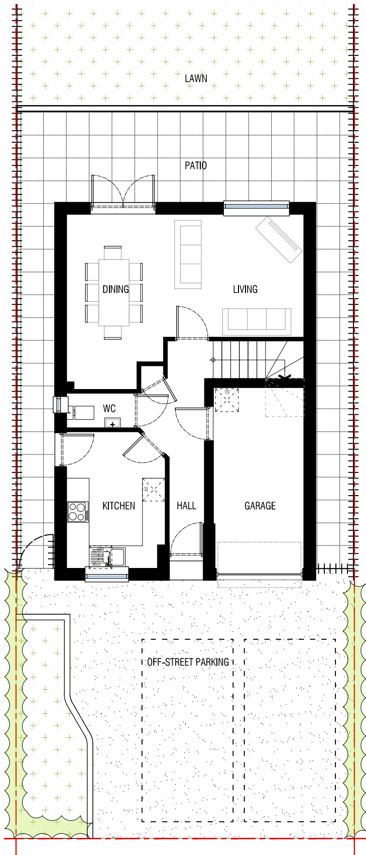
[01] EXISTING GROUND FLOOR PLAN 1:100
