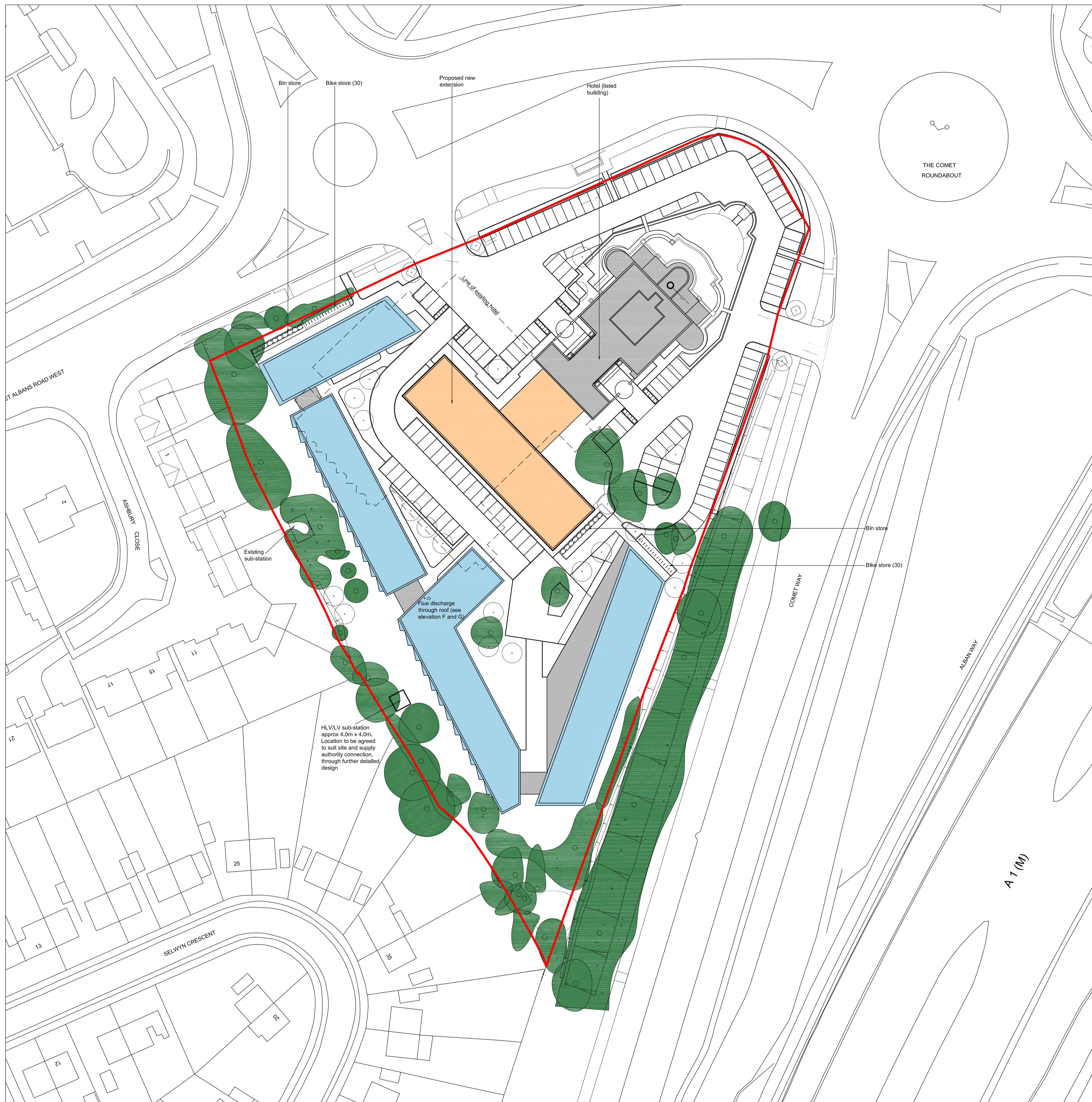
Roof Plan
