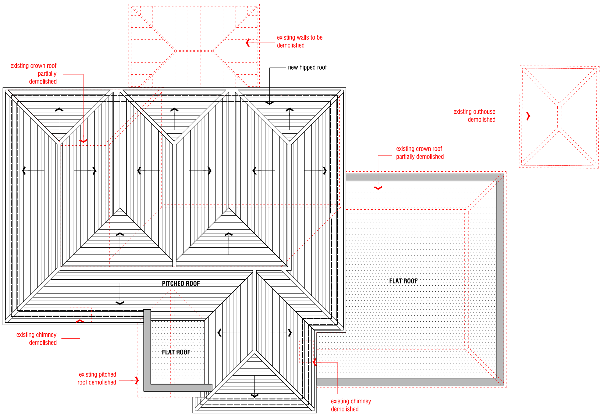
[01] EXISTING ROOF PLAN
