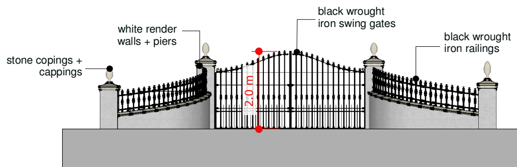
TYPICAL GATE ELEVATION 1:100
