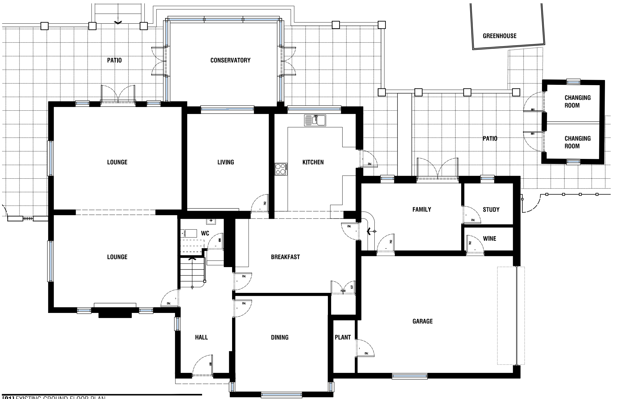
[01] EXISTING GROUND FLOOR PLAN
