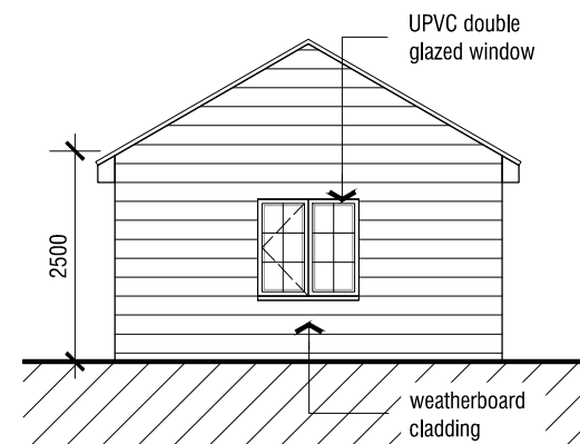
[04] PROPOSED SOUTHEAST ELEVATION (SIDE)
