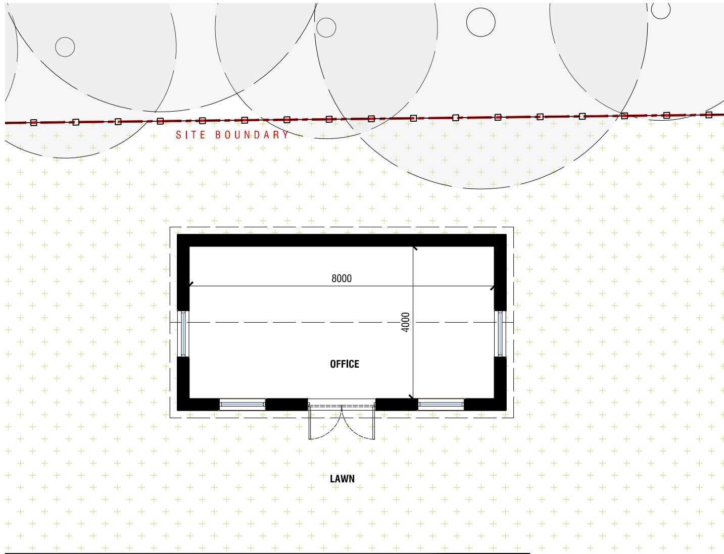
[01] PROPOSED OFFICE PLAN
