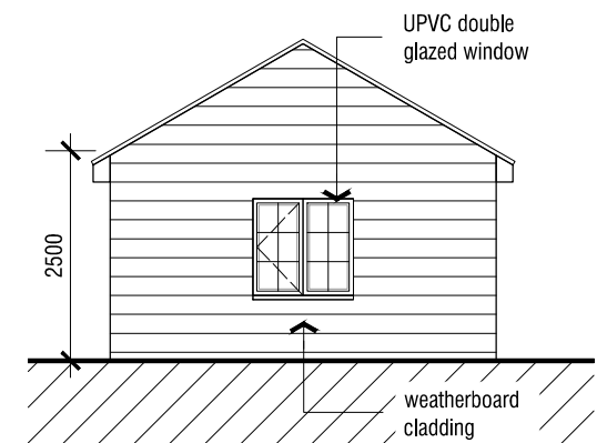
[05] PROPOSED NORTHWEST ELEVATION (SIDE)
