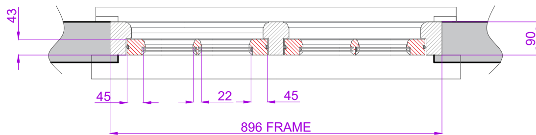
PLAN - SCALE 1:10
