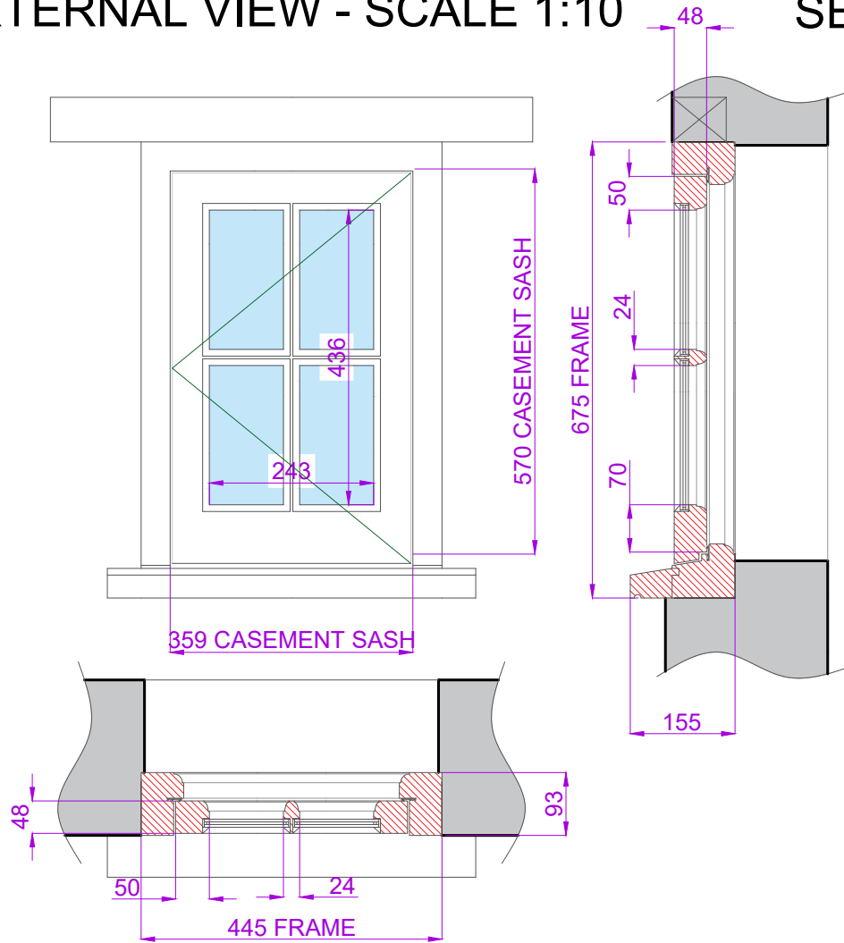
PLAN - SCALE 1:10
