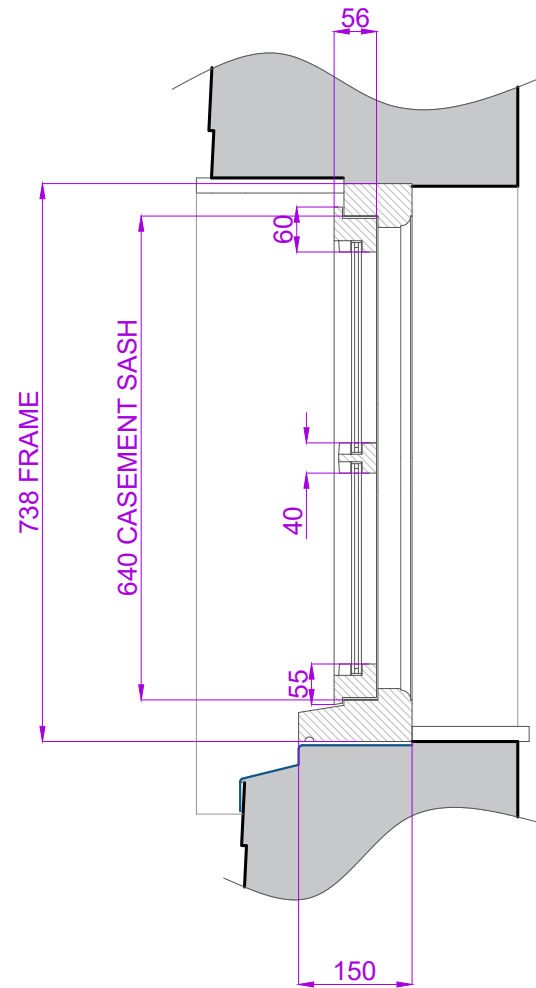
SECTION - SCALE 1:10
