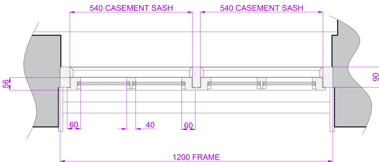
PLAN - SCALE 1:10
