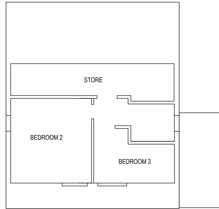
EXISTING FIRST FLOOR - 1:100
