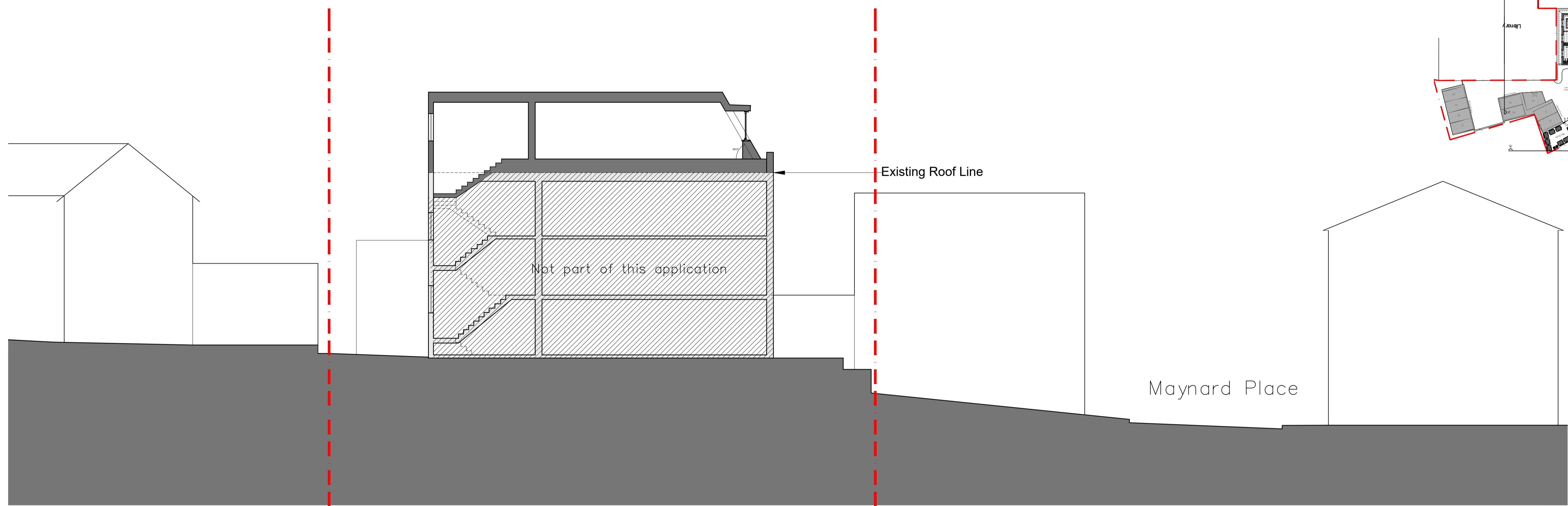
Proposed Section A-A 1:100 @A1 / 1:200 @A3
