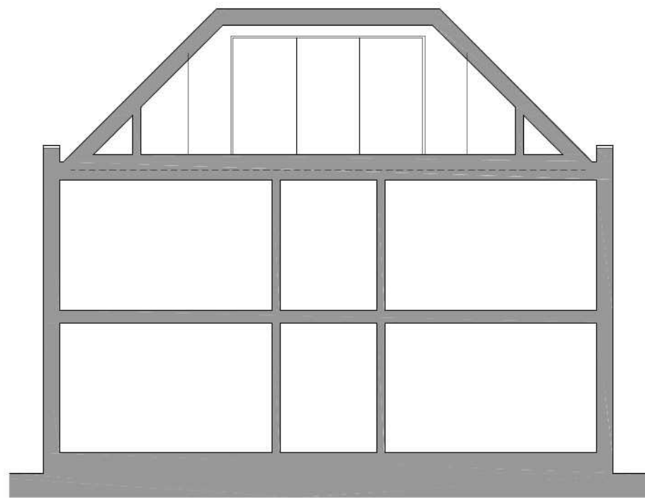
1 PROPOSED FRONT SECTION SK-008 SCALE@A1 1:50 SCALE@A3 1:100
