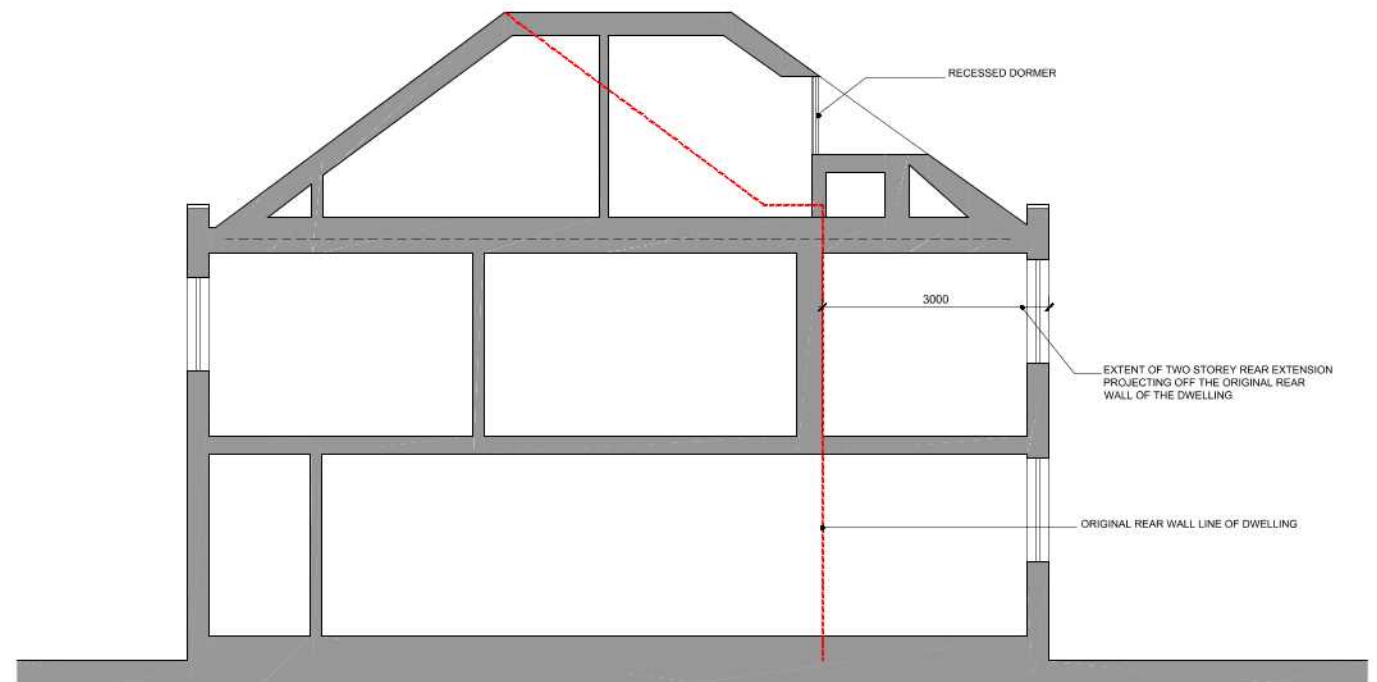
2 PROPOSED SIDE SECTION SK-008 SCALE@A1 1:50 SCALE@A3 1:100
