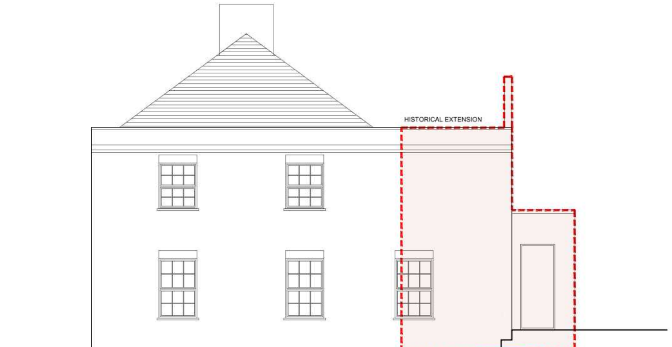
2 EXISTING SIDE 1 ELEVATION SK-004 SCALE@A1 1:50 SCALE@A3 1:100
