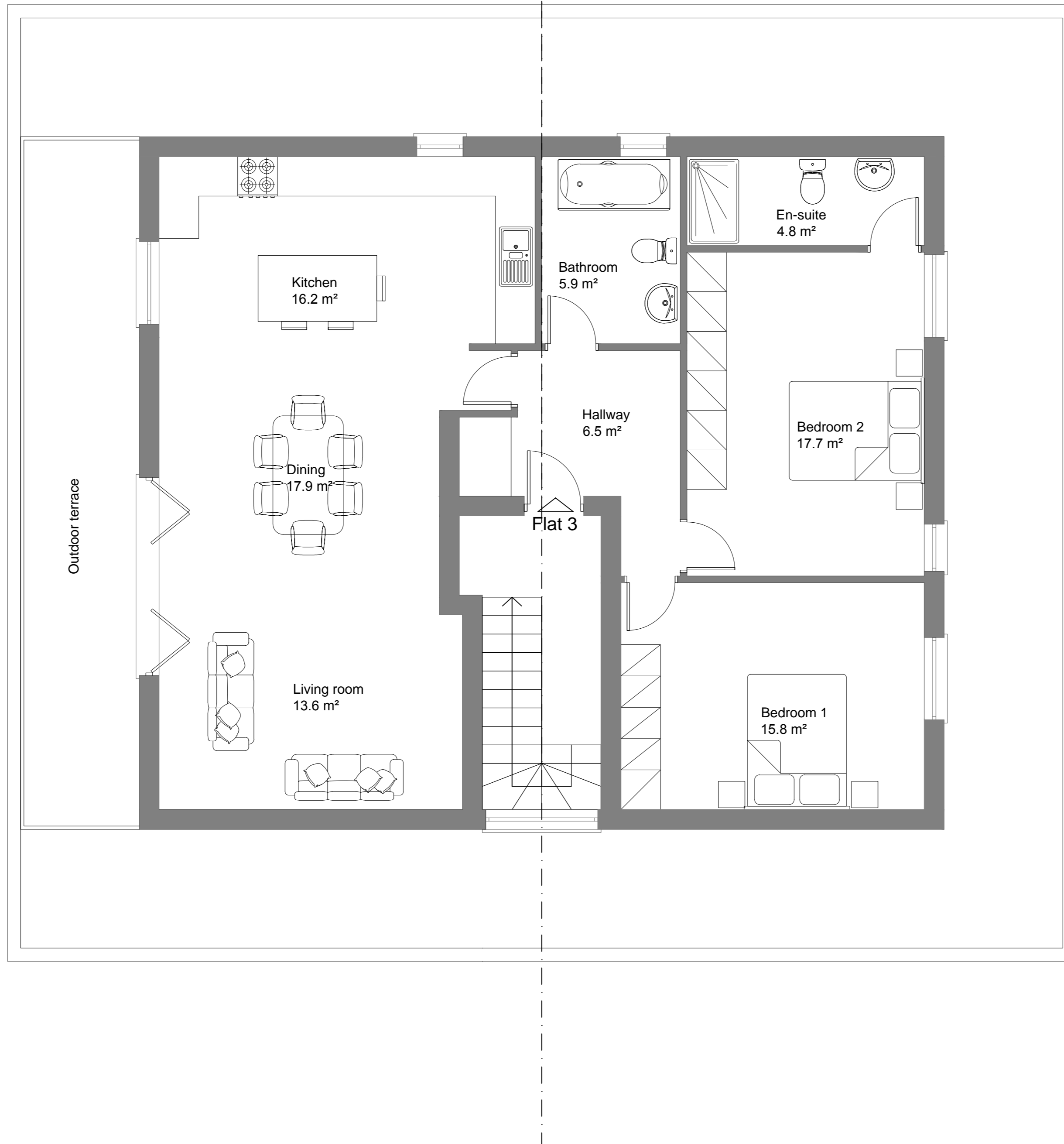
1 Proposed Second Floor Plan 1:50
