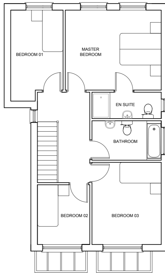
6 Proposed First Floor Plan 1:100
