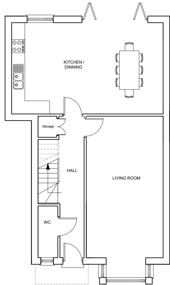
5 Proposed Ground Floor Plan 1:100
