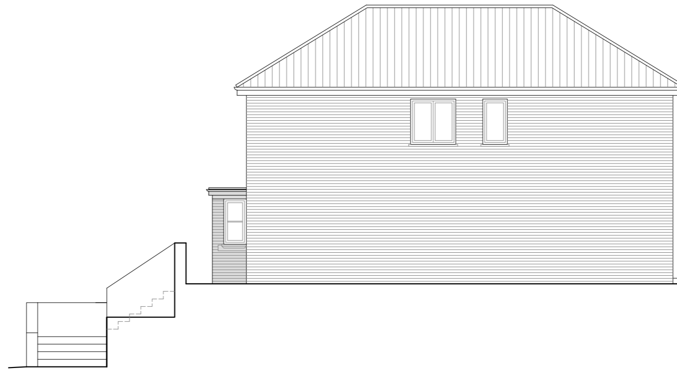
3 Proposed Side Elevation 1:100
