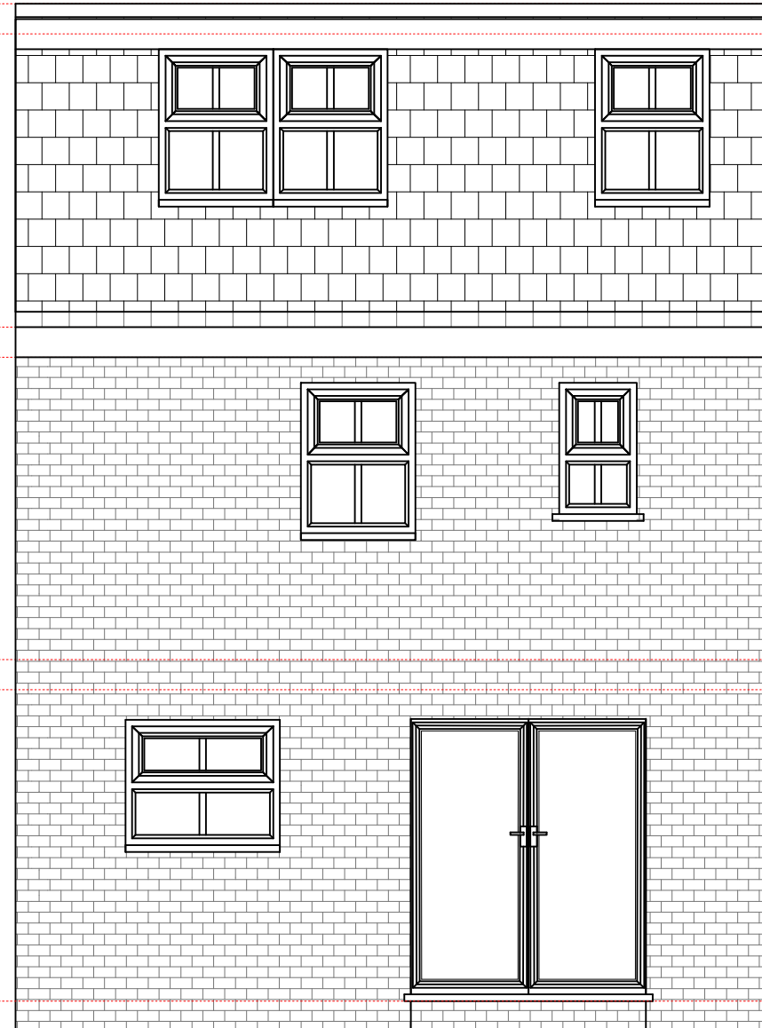
REAR ELEVATION [AS EXISTING]
