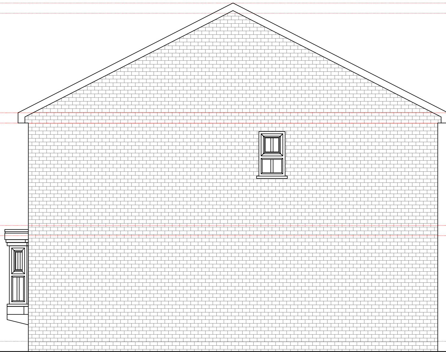
EAST FACING ELEVATION [AS EXISTING]
