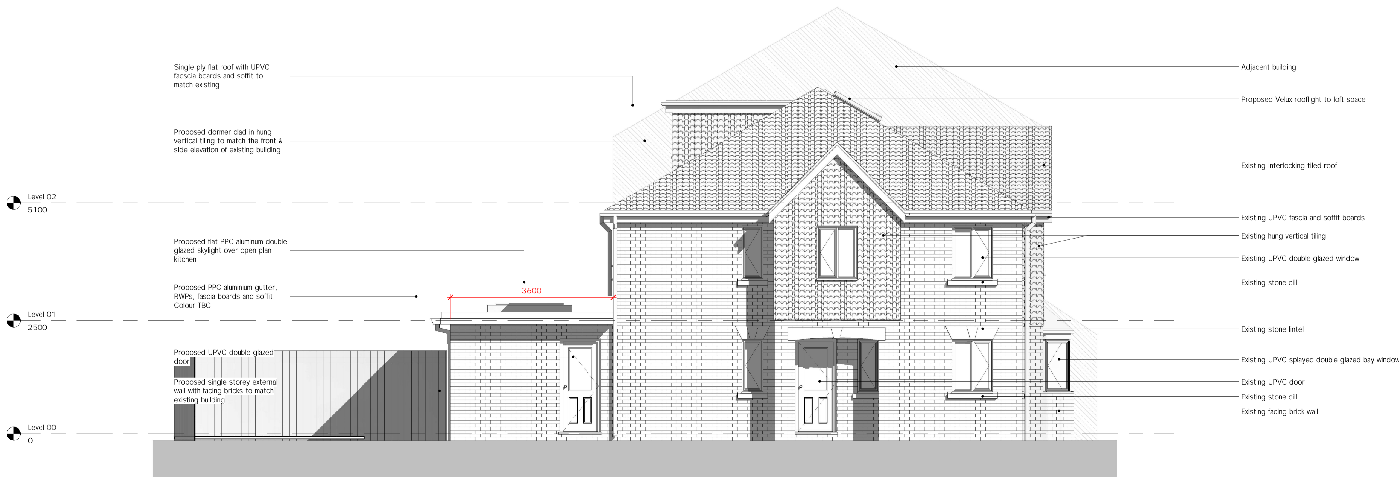
3 Proposed Side Elevation 1 : 50
