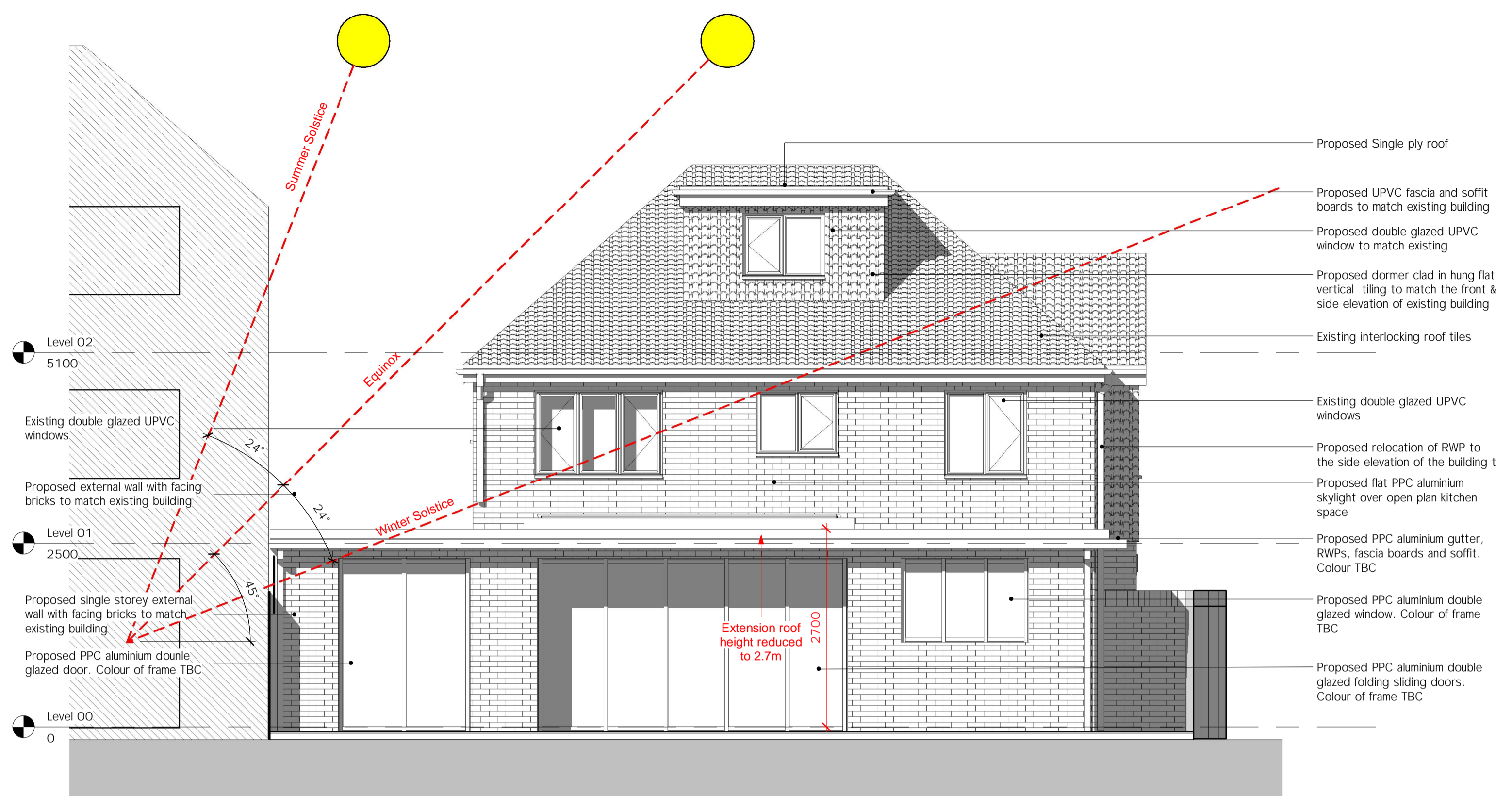
2 Proposed Rear Elevation 1 : 50
