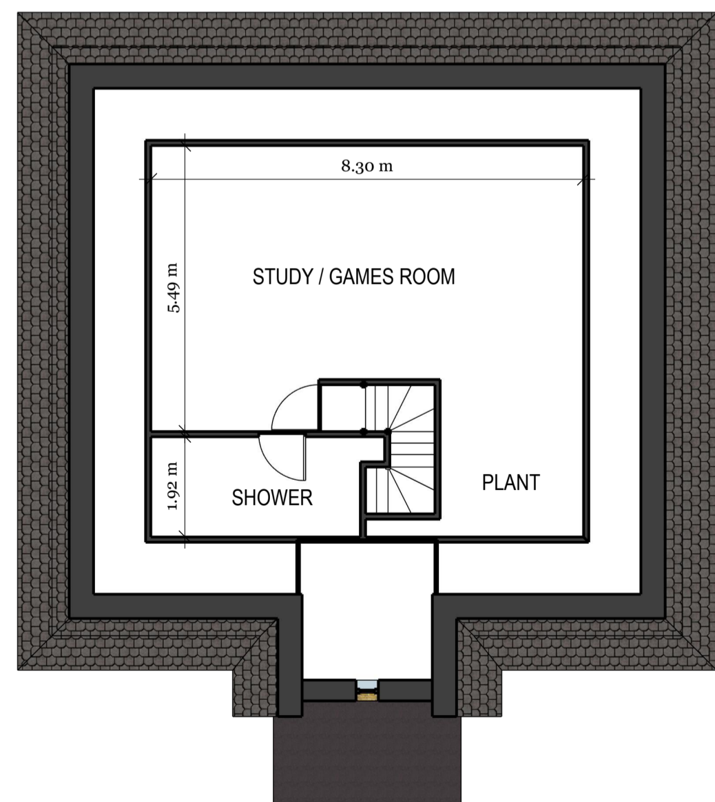
LOFT FLOOR PLAN scale: 1:100 G | 002
