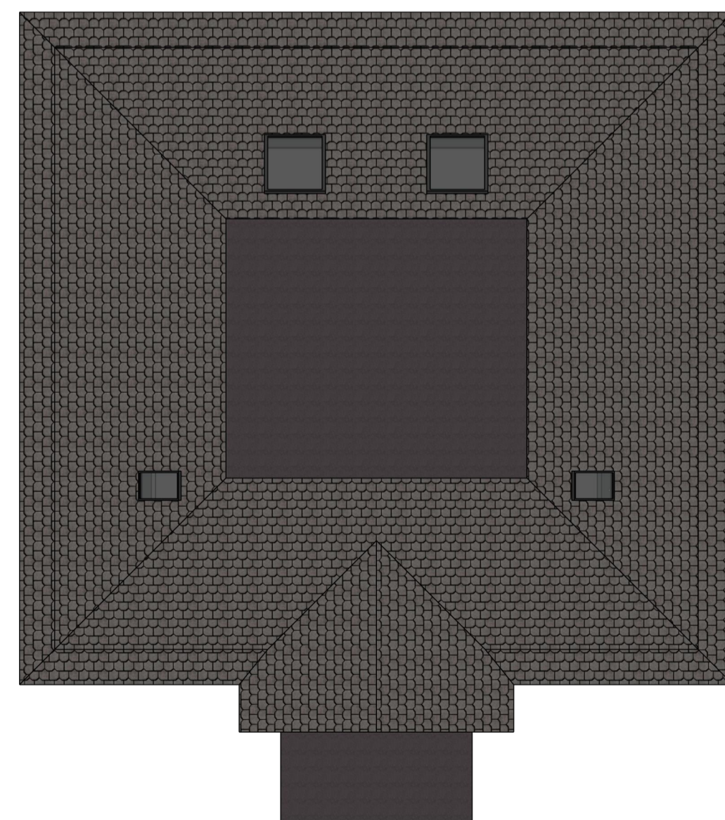
ROOF PLAN scale: 1:100 H | 002
