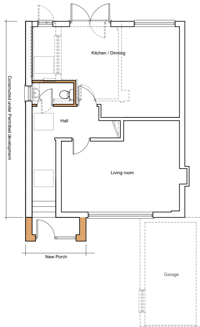
5 Proposed Ground Floor Plan 1:100
