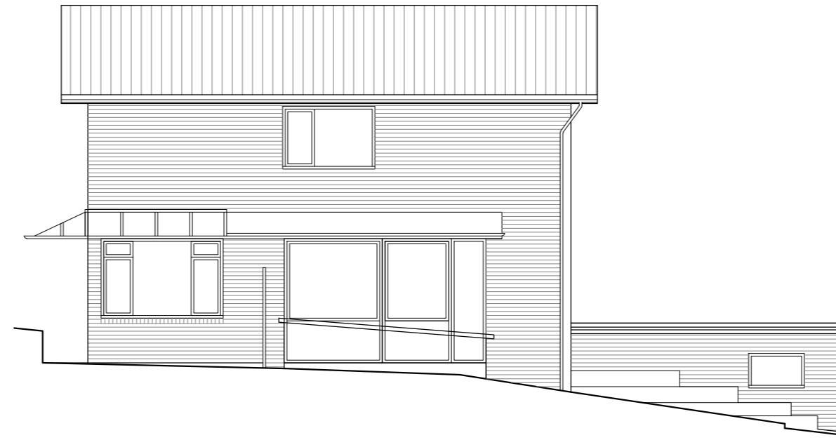
3 Existing Side Elevation 1:100
